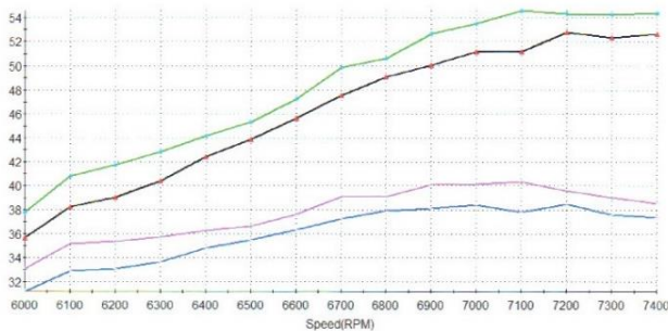
Figure 6: A-B dyno runs, same day. SlickCC AAPC coated 2 stroke pistons made approximately 7% more power across the rpm range
