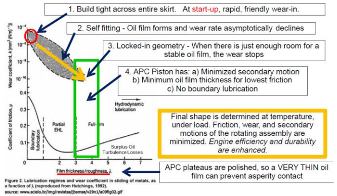
Figure 2: Stribeck Fitting Process 5
