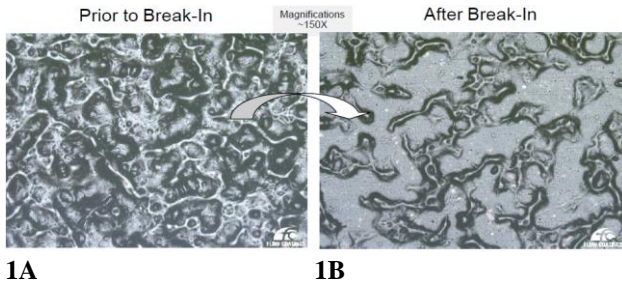
Figure 1A: Micro-photo “before” operation Figure 1B: Micro-photo “after” operation
