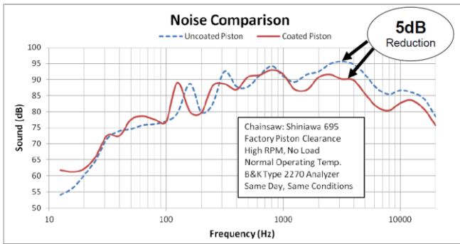
Figure 4B: SlickCC AAPC reduces Noise ~ 5db across audible spectrum
