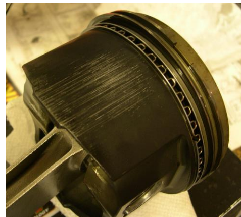
Figure 5C: AAPC protected this piston from ingested sand, and was used to restore the surface and resize the skirt for the newly honed bore dimension during overhaul. (Courtesy of Line2Line Coatings)
