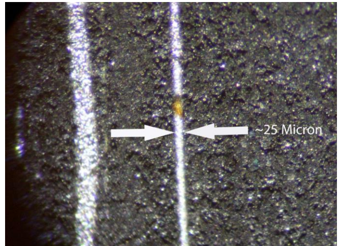
Figure 5B: Slick+ AAPC coated piston skirt with trapped crystallite particle
