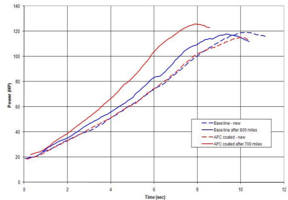
Figure 7B: A-B Acceleration 15% faster
