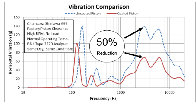
Figure 4A: Slick+ AAPC reduces Vibration
