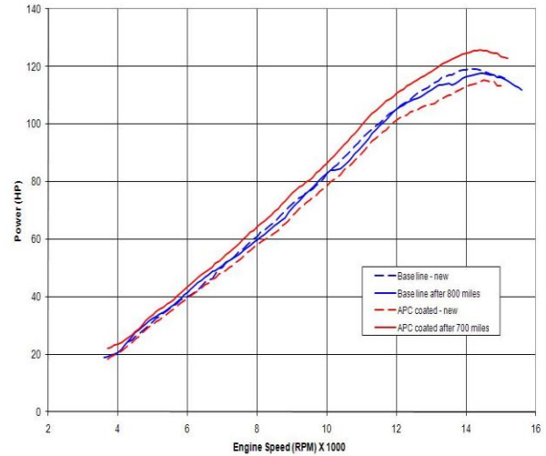
Figure 7A: A-B Peak HP 2% higher
